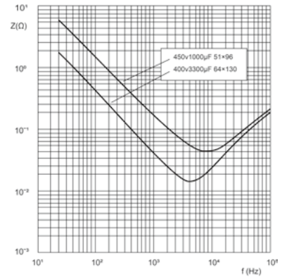
Impedance Z ~ Frequency at 20°C
